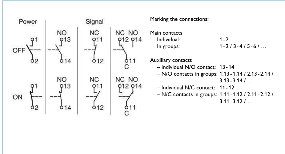
Fig. 17: Setting for auxiliary contacts based on switching state of the main contact
