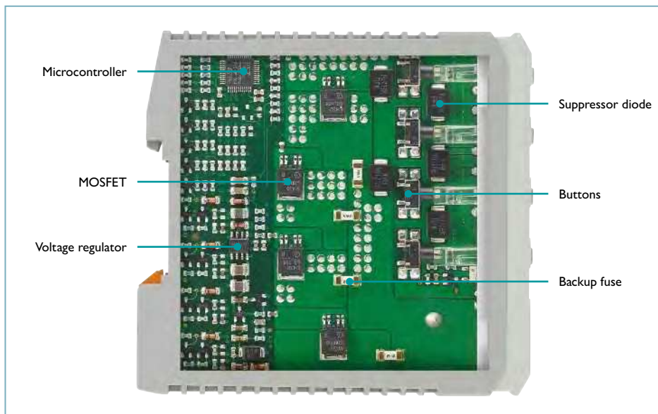
Fig. 15: Structure of a multichannel electronic circuit breaker
