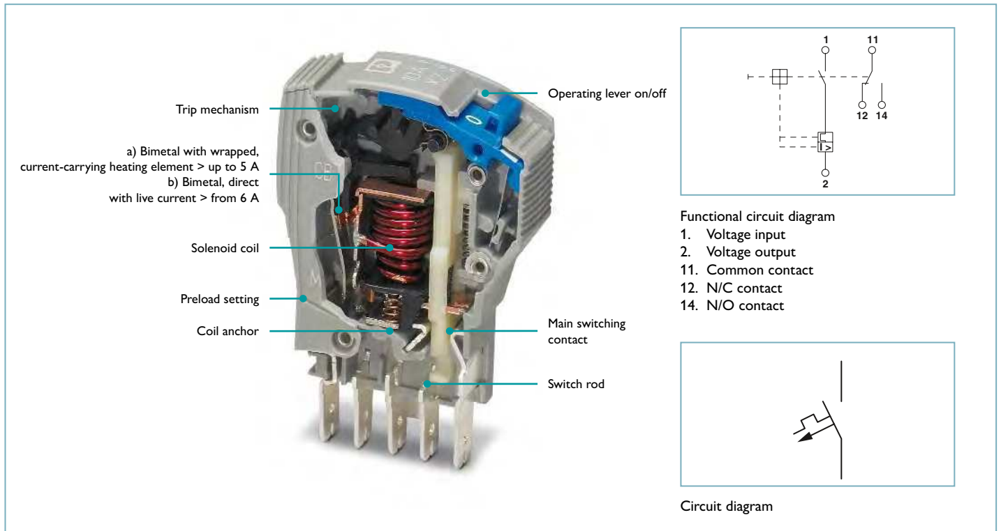
Fig. 10: Structure and functional description of thermomagnetic circuit breakers
