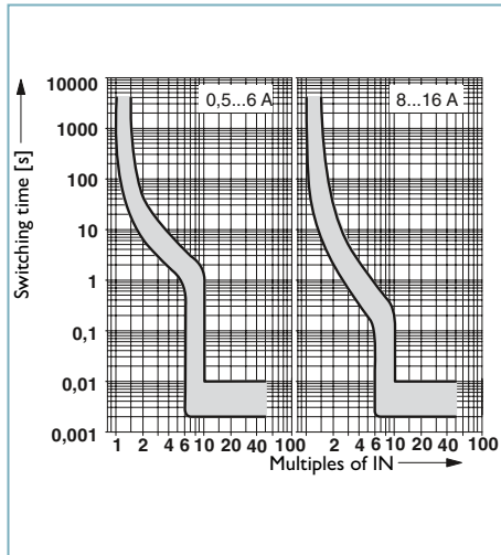
Fig. 12: SFB characteristic curve
